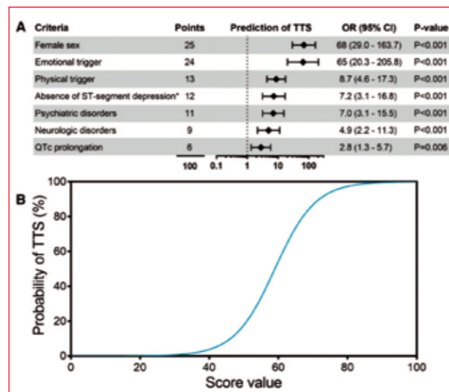
Figure 3. Score InterTAK 2 .
